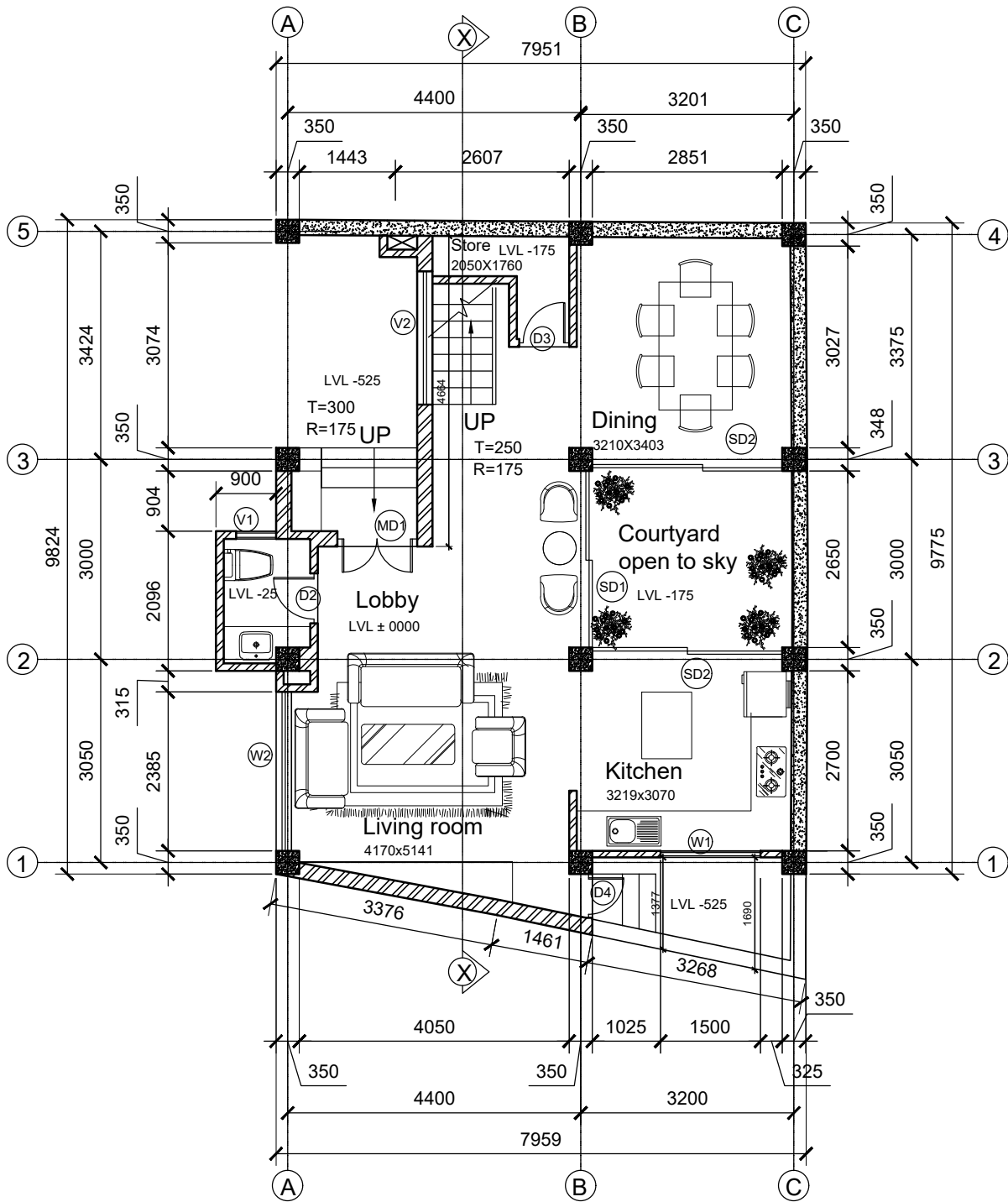
GROUND FLOOR PLAN C. Area: 73.53 sqm
